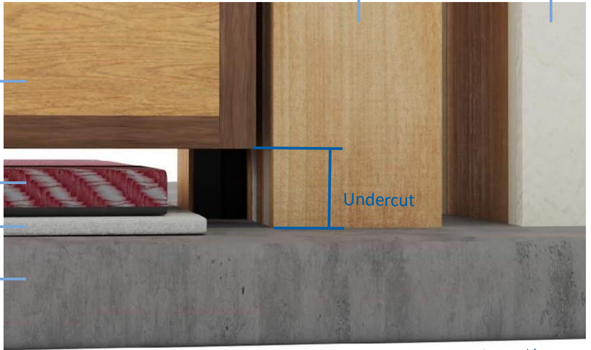
Bottom of the leaf and frame, showing undercut, floor finish and structural frame
